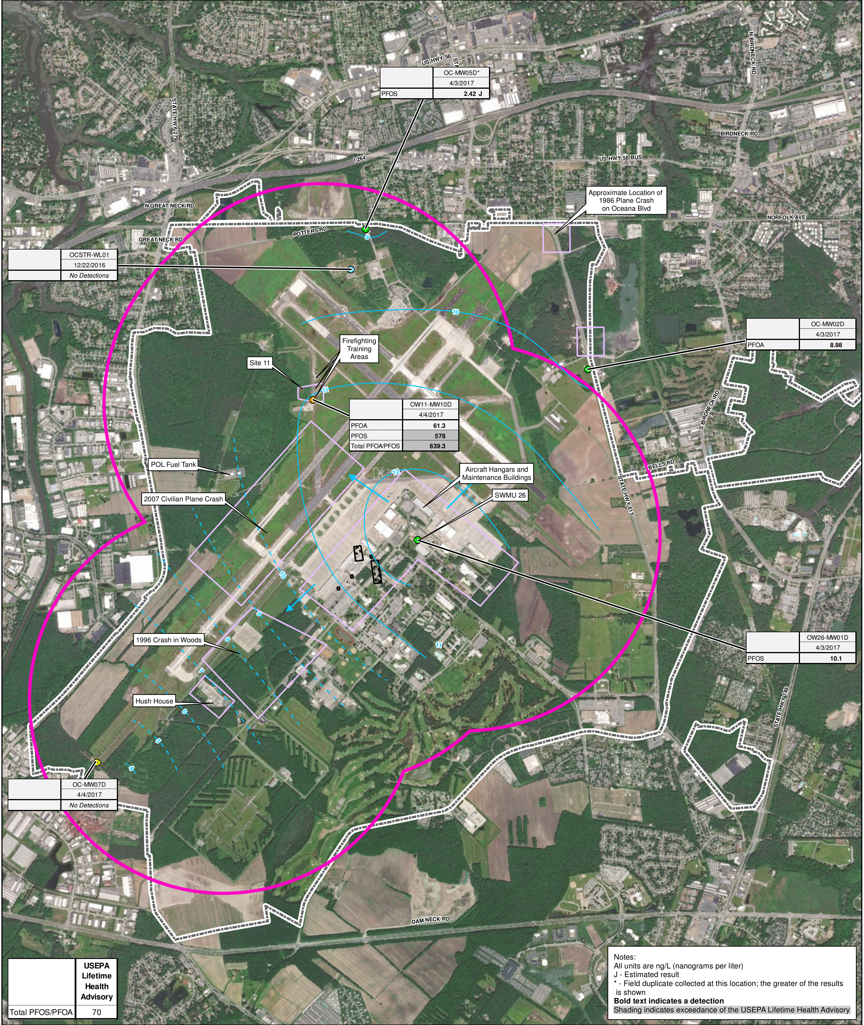
Figure 4-2 COCs Concentrations in the Yorktown Aquifer Basewide Per- and Polyfluoroalkyl Substances Site Inspection Report NAS Oceana, Virginia Beach, Virginia
